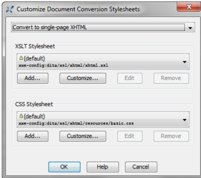
Figure 9.17. The "Customize Document Conversion Stylesheets" dialog box showing the stylesheets used when a DITA map is converted to single-page XHTML
